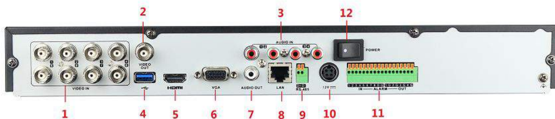
Figure 1. 4 Rear Panel
